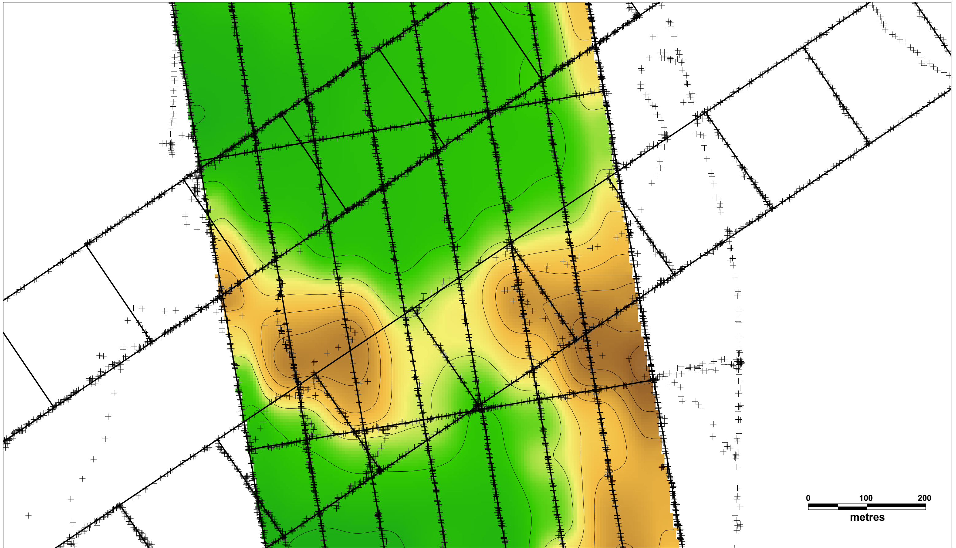
ARCHER LEVELLED TRACK POINTS (UNFILTERED) WITH DGPS GRIDDED ELEVATION DATA
