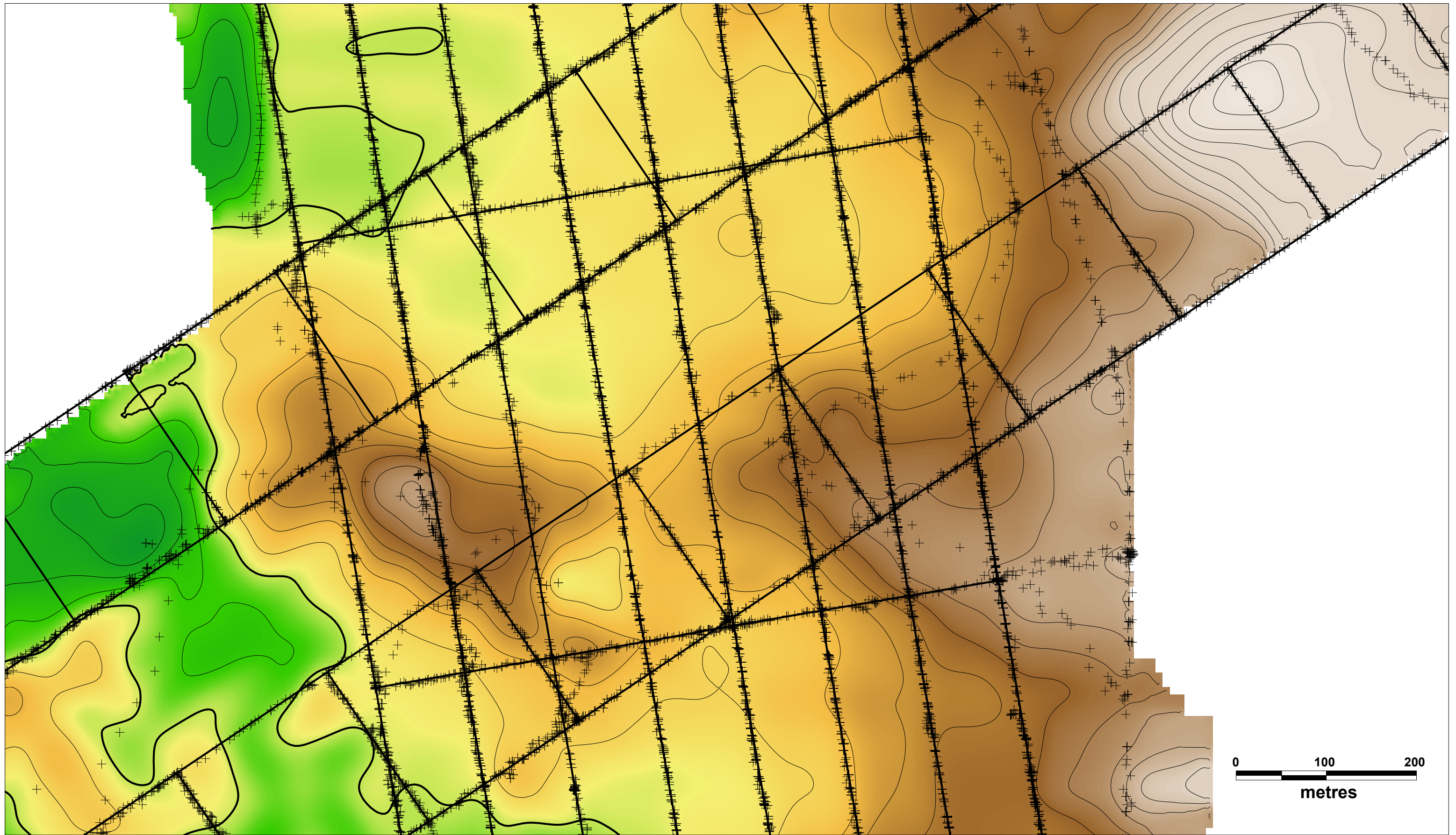
ARCHER LEVELLED TRACK POINTS (UNFILTERED) WITH GRIDDED ELEVATION MODEL
